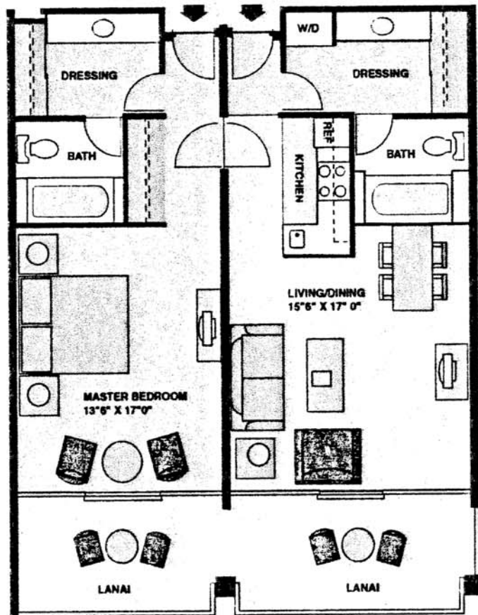
One-bedroom 1091 total sq. ft.
